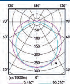
WT120C G2 schaltbar
