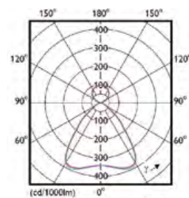
SP342P, PCS, BAP-tauglich
