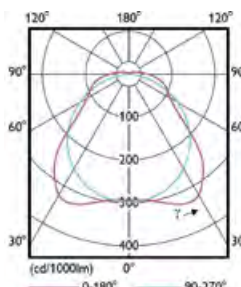
WT120C G2 PSD / PSU MDU
