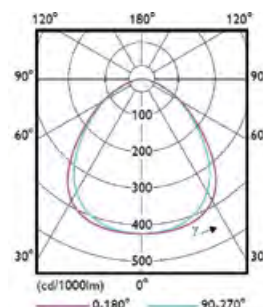
RC132V G4 / RC133V G4 OC, BAP-tauglich
