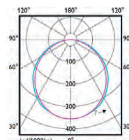
SM531C, opal
