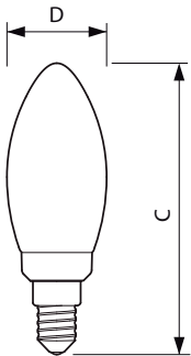
B35 230V 6-40W 470lm 2700-2200K E14 D CL
